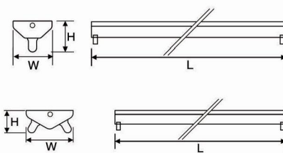
Ballast: LD55
